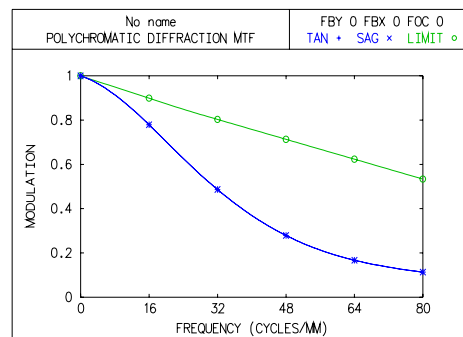
Fig. 6. Arizona model
