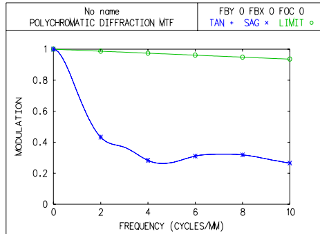
Fig. 3. Emsley model
