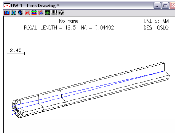
Fig. 2. Arizona model (3D solid facets)
