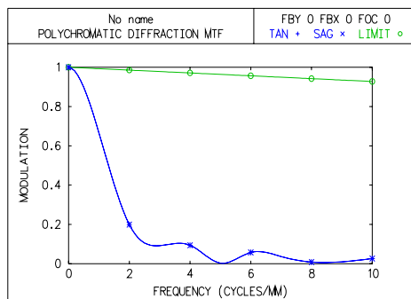
Fig. 5. Liou-Brennan model
